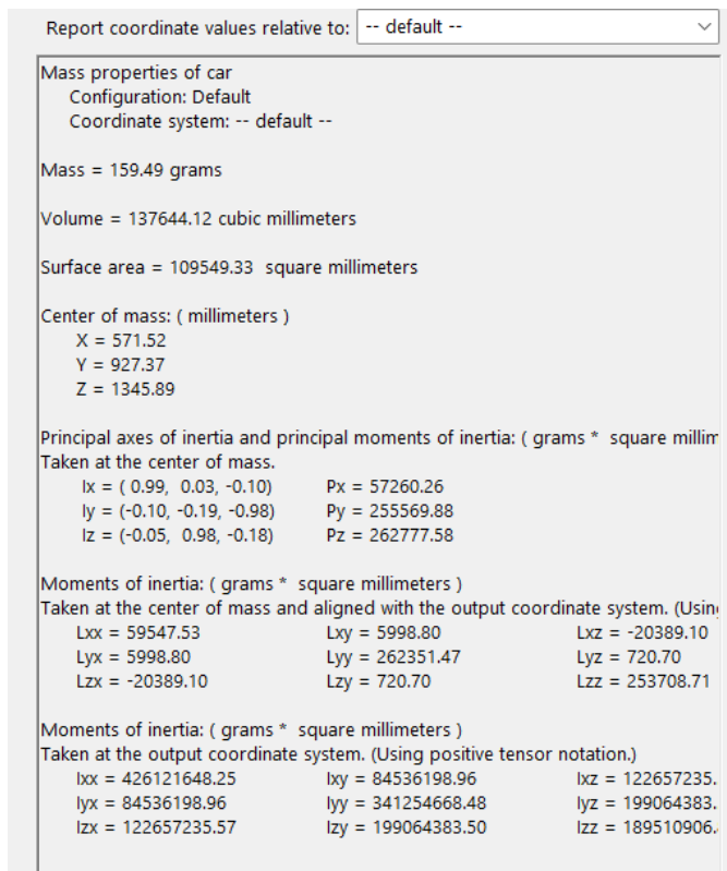
Figure 6: Mass properties of the 'Blue' car
